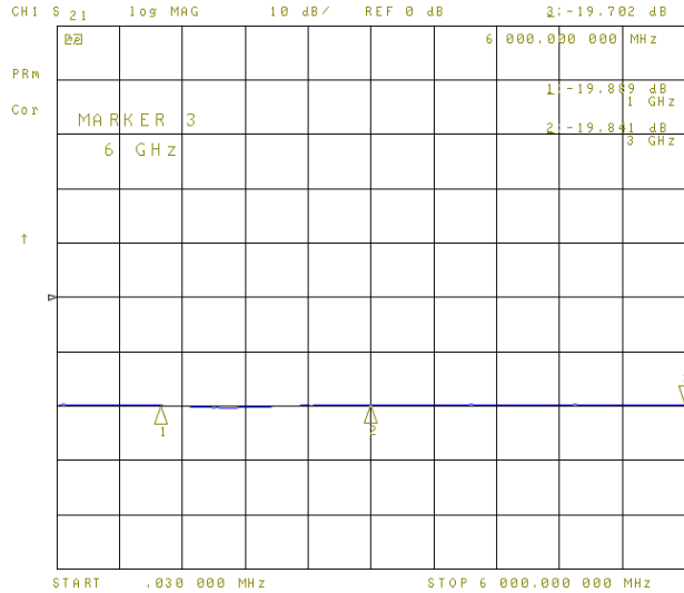
20dB Attenuator, S21
