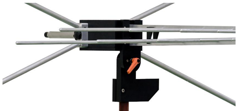
Optional TBMA8-PA mounting bracket; only recommended for setups with limited space
