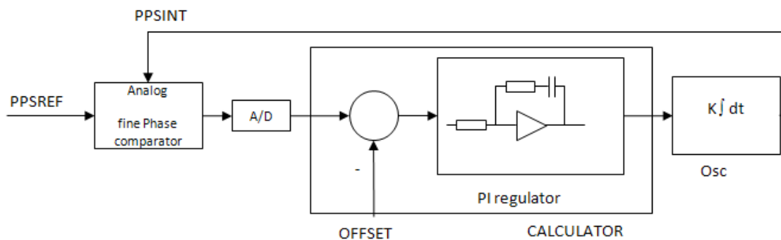
Figure 6 schematic of the analog fine phase comparator regulation loop
