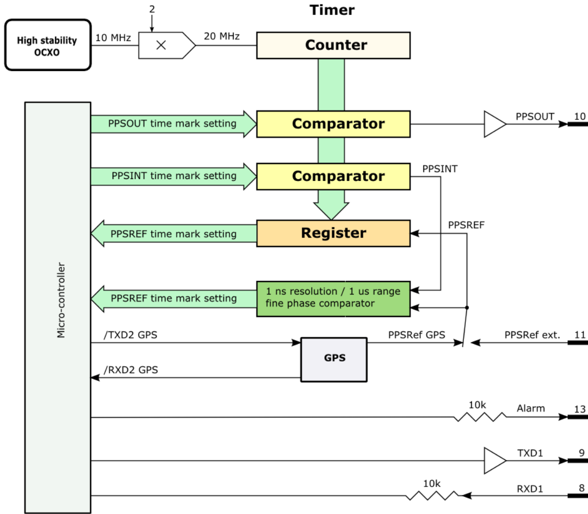
Figure 2 Timing system.
