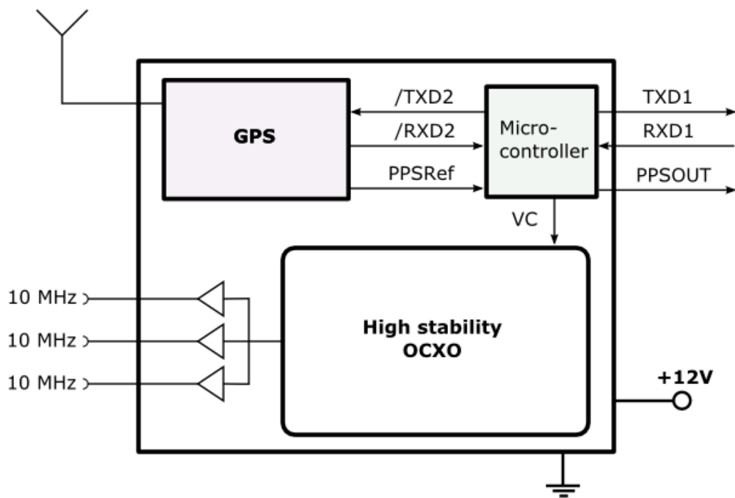
Figure 1 Building block of the GXClock-500
