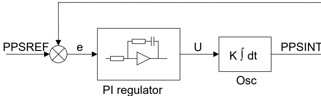
Figure 4 Schematic of the PPSREF regulation loop.
