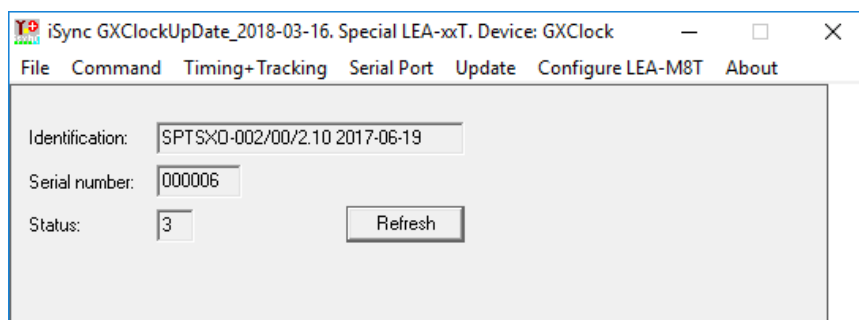
Figure 1 - GxClock Manager.exe
