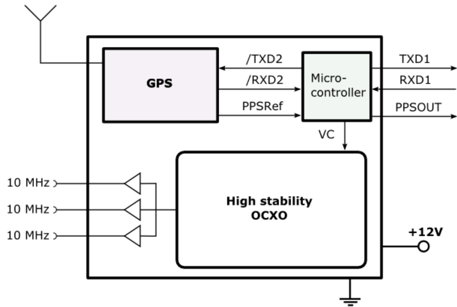
Figure 2: Building block of the GXClock-500 module inside the GNSSource-1000
