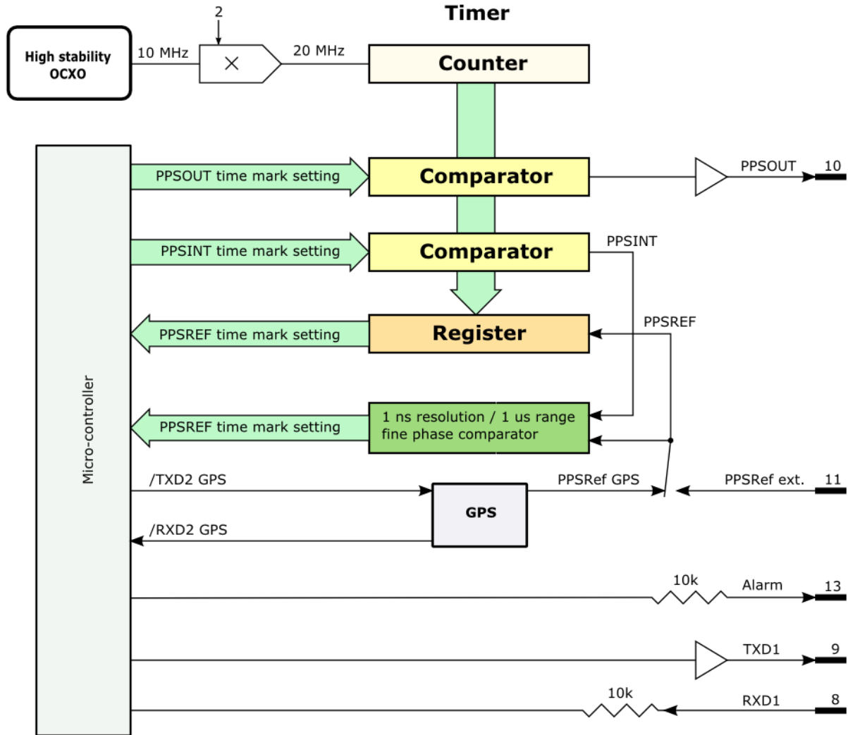
Figure 3: Timing system.
