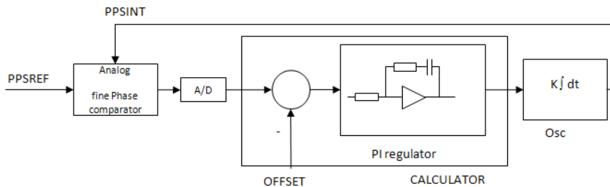
Figure 7 schematic of the analog fine phase comparator regulation loop
