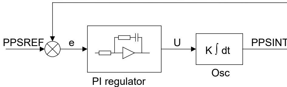
Figure 5: Schematic of the PPSREF regulation loop.
