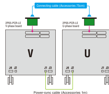
[Example of single phase 3-wire 4 kVA system]
