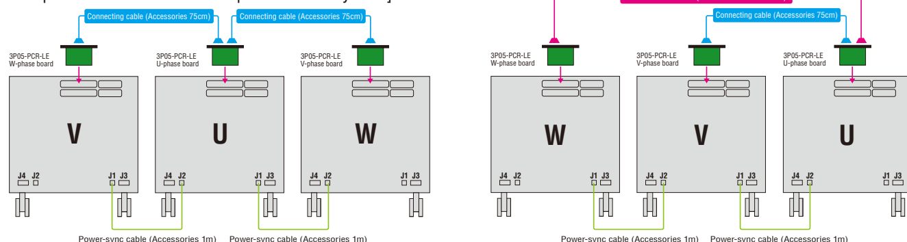
[Example of PCR2000LE Three phase 6 kVA system]
