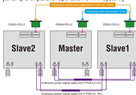
[Example of parallel operation 6 kVA system]
