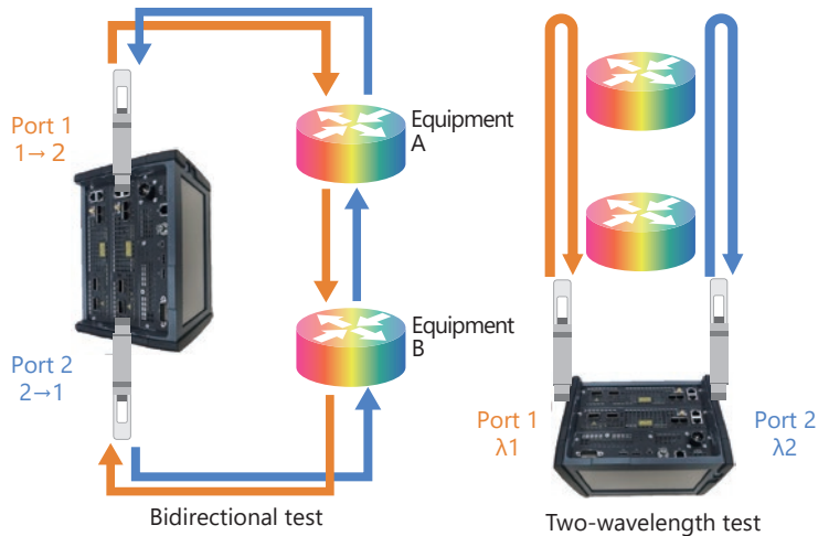
Example of 2-port independent test
